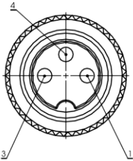
Positions of contacts
