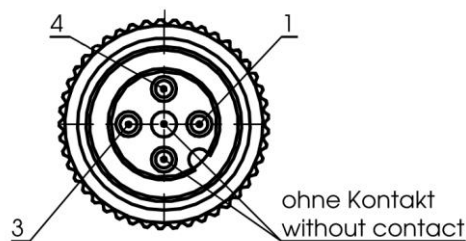
Positions of contacts
