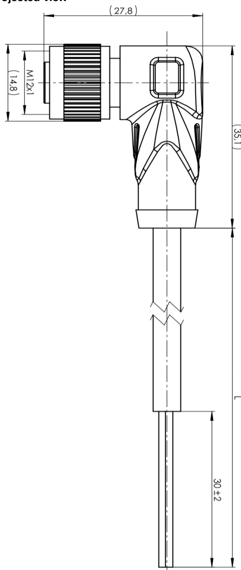
Projected view
