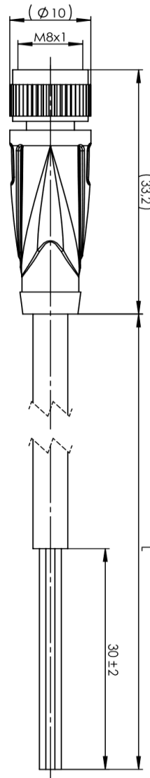
Projected view
